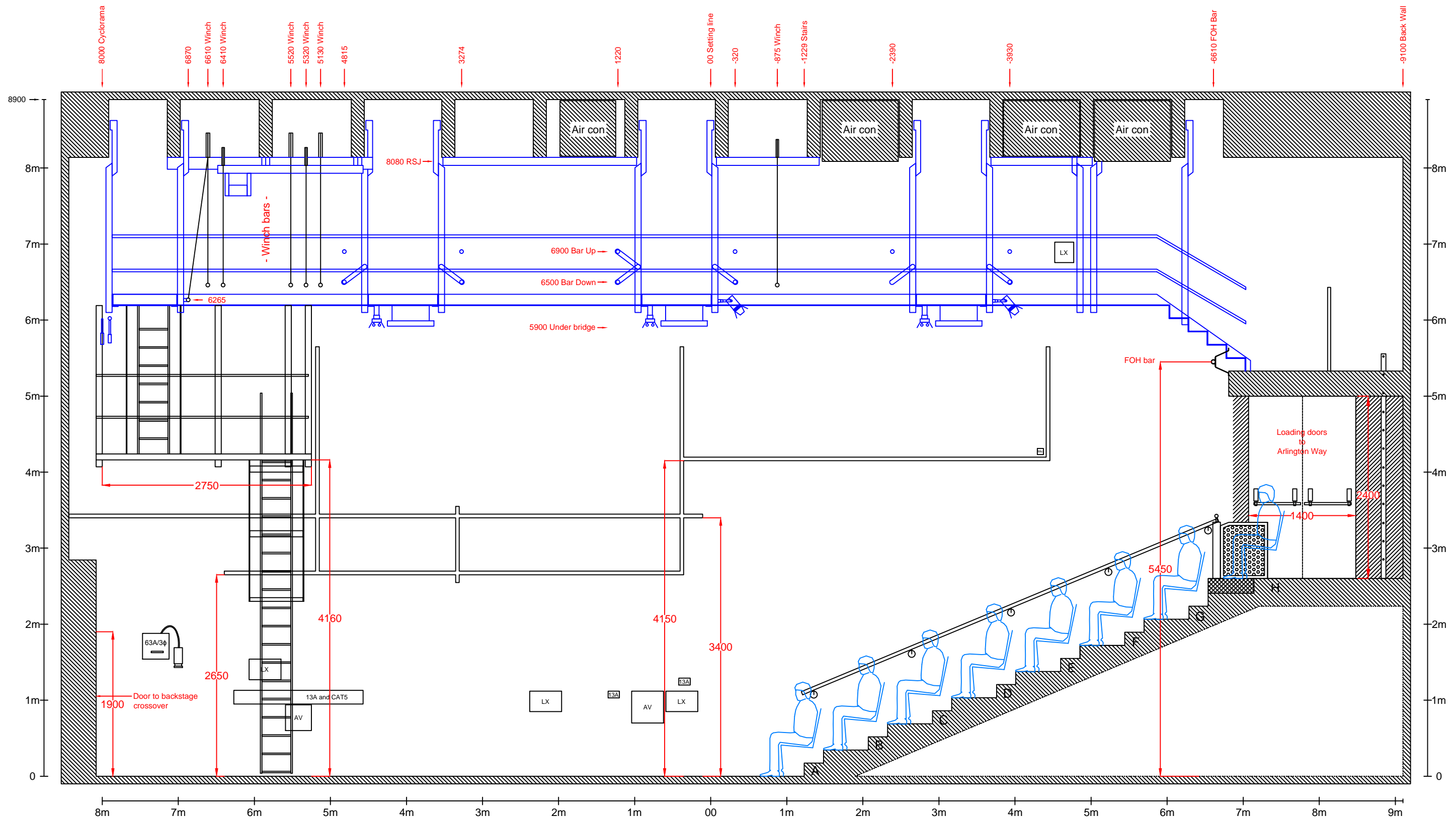
STAGE LEFT WALL PLAN
